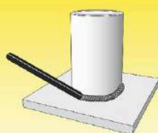
Pipe fixed with axis vertical: PB/2F
